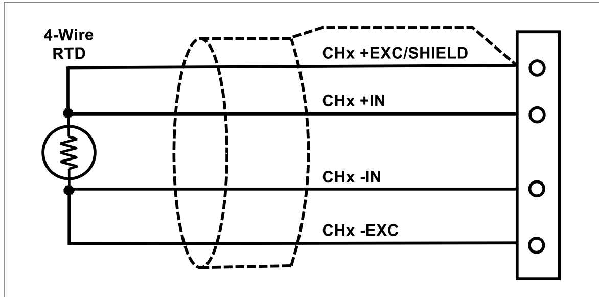
Figure 5: MAQ20-RTD41 4-Wire RTD Sensor Wiring
