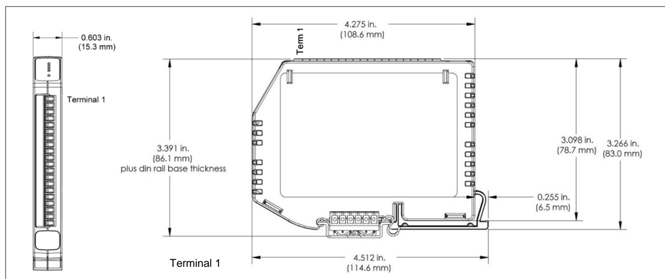
Figure 1: Module Dimensions
