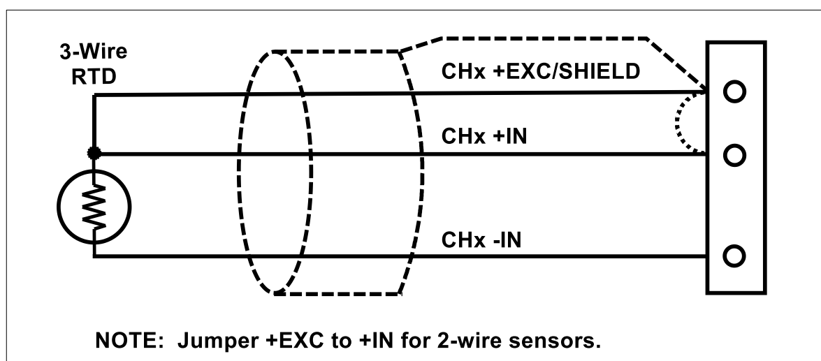
Figure 2: MAQ20-RTD31 3-Wire and 2-Wire RTD Sensor Wiring
