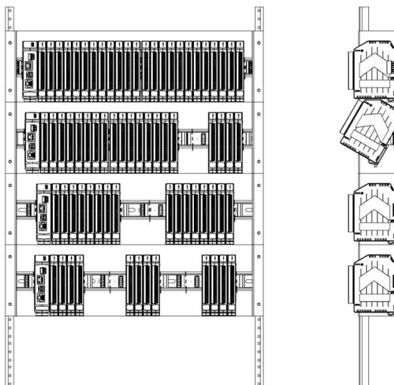
Figure 7: Possible System Configurations
