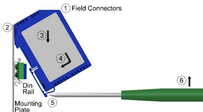
Figure 6: Module Installation and Removal
