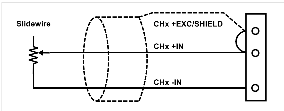
Figure 4: MAQ20-RTD31 Slidewire Sensor Wiring
