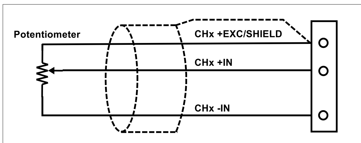
Figure 3: MAQ20-RTD31 Potentiometer Sensor Wiring
